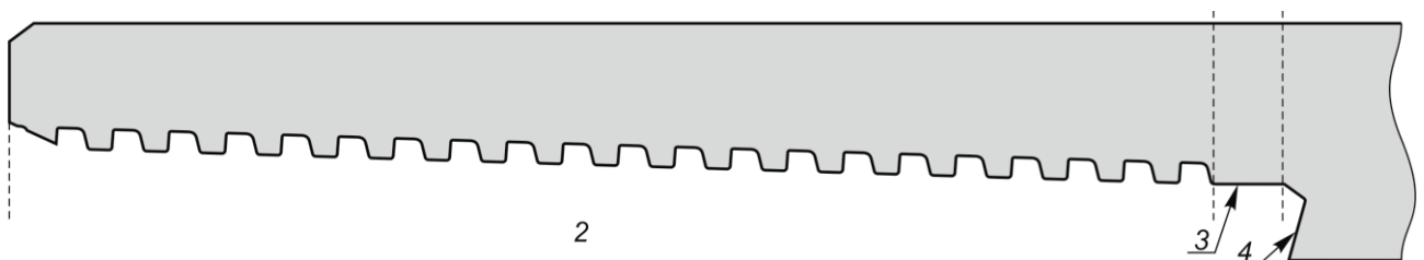
b) – Surface of internal thread connection
