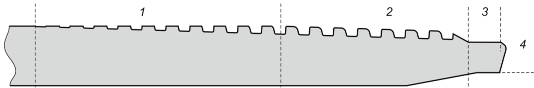
a) – Surface of external thread connection
