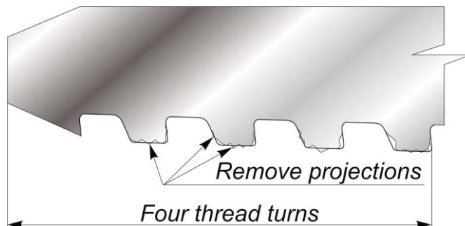
b) – Surface of internal thread connection
