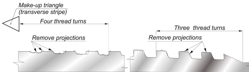
a) – Surface of external thread connection
